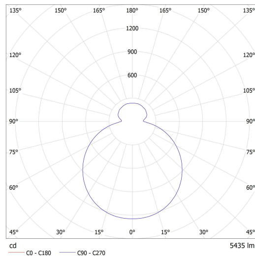
Lucis PS13.K2.Z600 ZERO LED / LDC (Polar)
