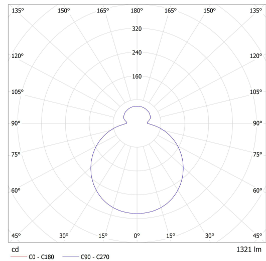
Lucis PS13.K3.Z330 ZERO LED / LDC (Polar)
