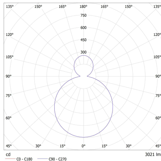
Luminaire: Lucis PS13.K1.R550 RONDO LED Lamps: 1 x LED G5
