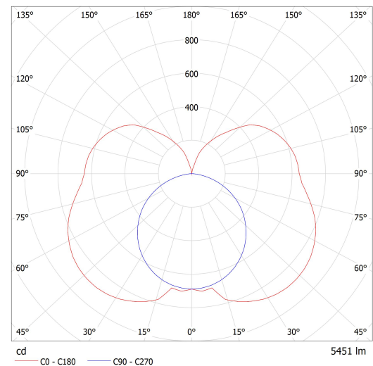
Luminaire: Lucis ZLI3.L2.1200.X IZAR III LED Lamps: 1 x LED G6
