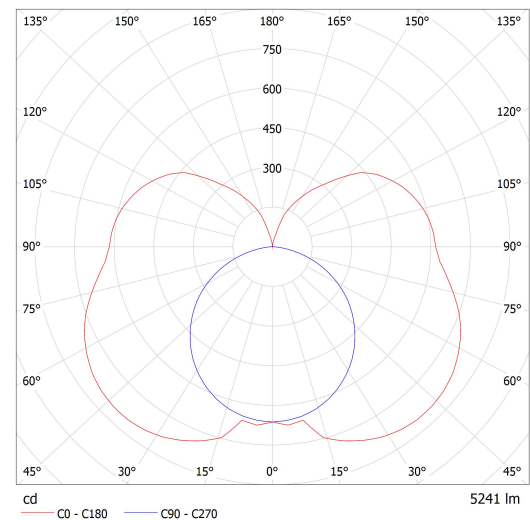
Luminaire: Lucis ZLI3.L1.1200.X IZAR III LED Lamps: 1 x LED G6
