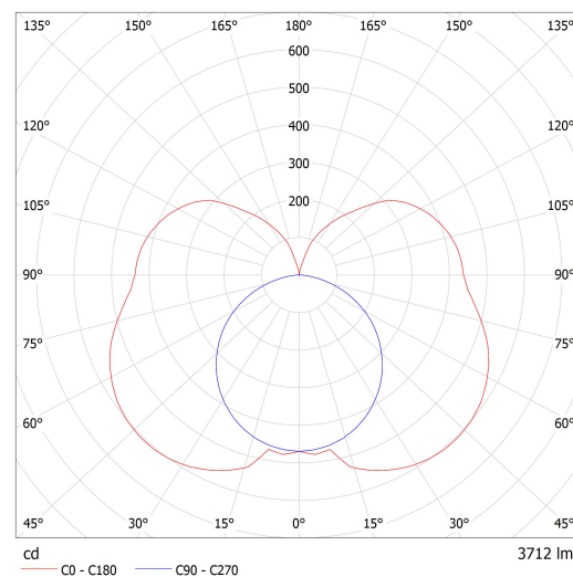
Luminaire: Lucis ZLI3.L1.900.X IZAR III LED Lamps: 1 x LED G6
