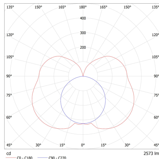
Luminaire: Lucis ZLI3.L2.600.X IZAR III LED Lamps: 1 x LED G6
