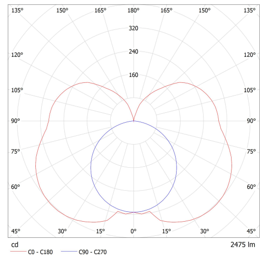
Luminaire: Lucis ZLI3.L1.600.X IZAR III LED Lamps: 1 x LED G6
