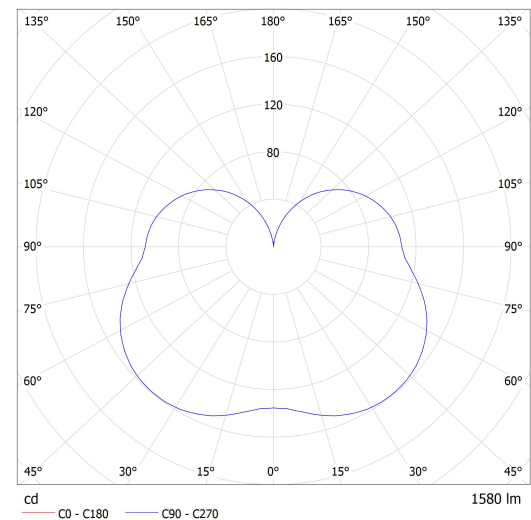
Luminaire: Lucis ZL1.IC.L2.330.X IZAR C LED Lamps: 1 x LED 2987
