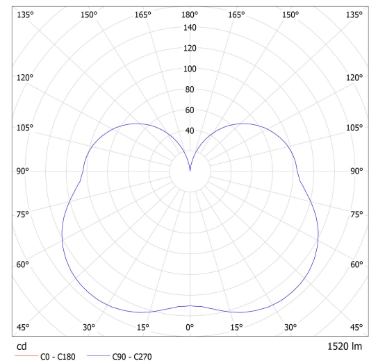
Luminaire: Lucis ZL1.IC.L1.330.X IZAR C LED Lamps: 1 x LED 2985
