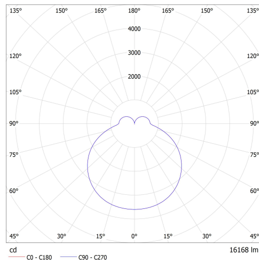
Lucis IB.L2.900M.X IZAR B MAX LED / LDC (Polar)
