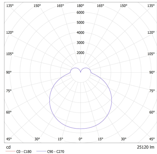
Lucis IB.L2.1250M.X IZAR B MAX LED / LDC (Polar)
