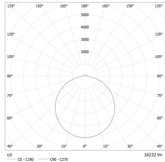
Lucis IB.L1.900.X IZAR B LED / LDC (Polar)
