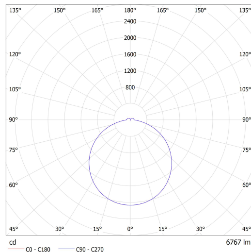
Lucis IB.L1.600.X IZAR B LED / LDC (Polar)
