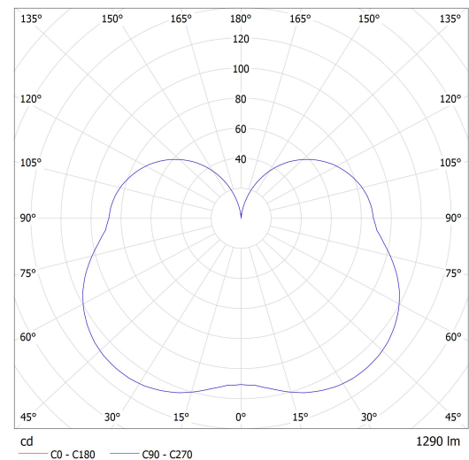
Luminaire: Lucis ZL1.IC.L2.250.X IZAR C LED Lamps: 1 x LED 2950 G4
