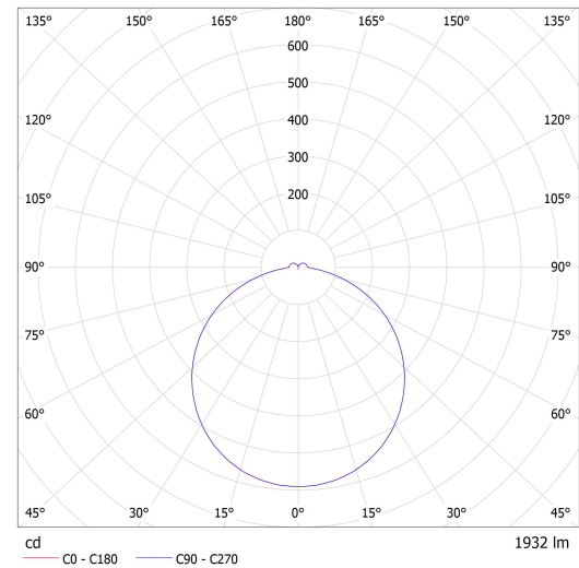
Lucis IB.L1.330.X IZAR B LED / LDC (Polar)
