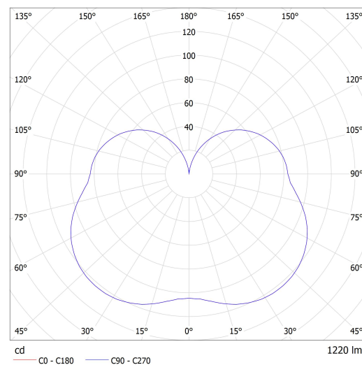
Luminaire: Lucis ZL1.IC.L1.250.X IZAR C LED Lamps: 1 x LED 2949 G4
