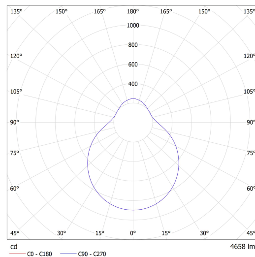
Luminaire: Lucis ZT.L2.D550.X DAPHNE LED Lamps: 1 x LED G6
