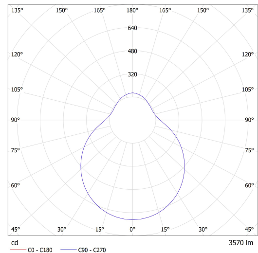
Luminaire: Lucis ZT.L1.D450.X DAPHNE LED Lamps: 1 x LED G6
