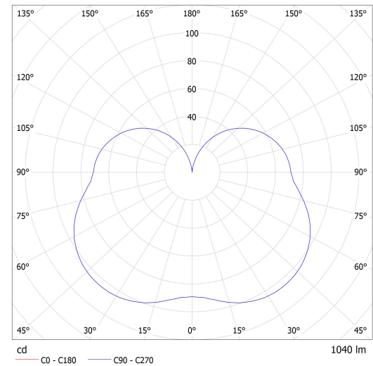
Luminaire: Lucis ZL1.IC.L2.150.X IZAR C LED Lamps: 1 x LED 2909
