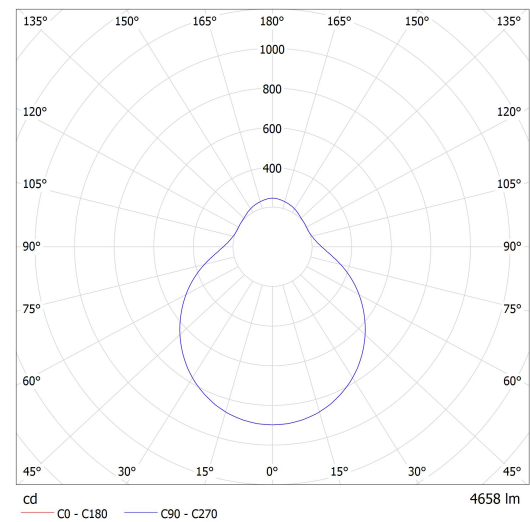
Luminaire: Lucis PS13.L2.D550 DAPHNE LED Lamps: 1 x LED G6
