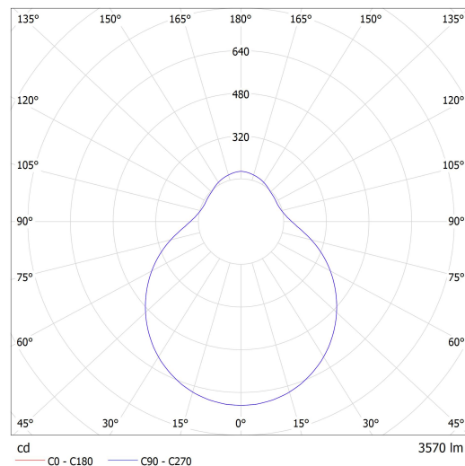
Luminaire: Lucis PS13.L1.D450 DAPHNE LED Lamps: 1 x LED G6
