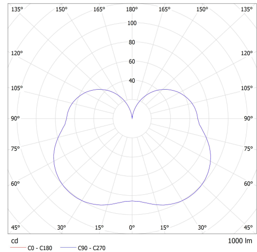
Lucis ZL1.IC.L1.150.X IZAR C LED / LDC (Polar)
