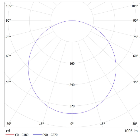
Lucis O.525.K2.X OMNIA LED / LDC (Polar)
