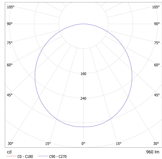
Luminaire: Lucis O.1250.K1.X OMNIA LED Lamps: 1 x LED G5
