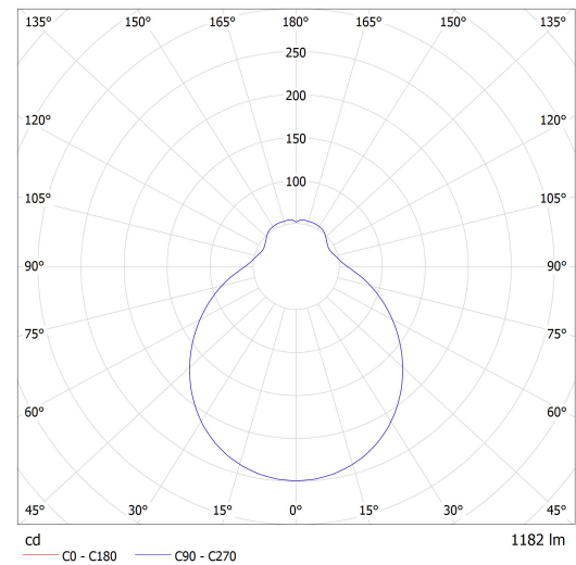
Luminaire: Lucis S24.L4.T12 CHARON LED Lamps: 1 x LED G6
