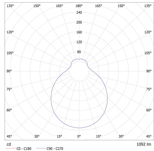
Luminaire: Lucis S24.L3.T12 CHARON LED Lamps: 1 x LED G6
