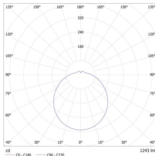
Luminaire: Lucis S26.L4.CA2 CHARON PMMA LED Lamps: 1 x LED G6
