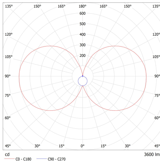
Lucis I2.L1.900.X IZAR II LED / LDC (Polar)
