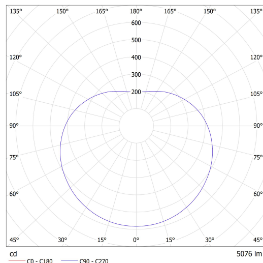
Luminaire: Lucis ZL1.P1.500.X POLARIS ZL LED Lamps: 1 x LED G6
