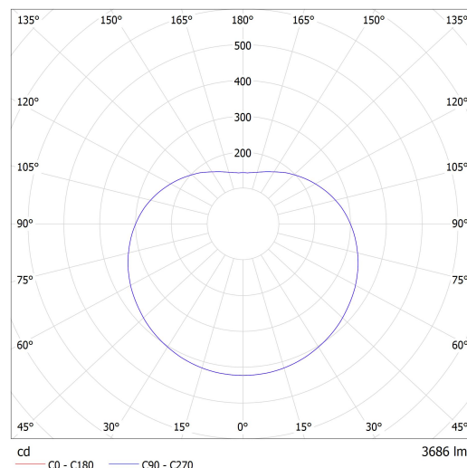
Luminaire: Lucis ZL1.P2.400.X POLARIS ZL LED Lamps: 1 x LED G6
