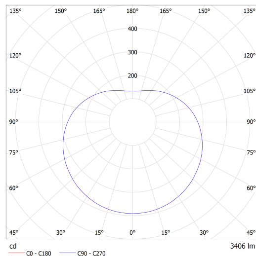
Luminaire: Lucis ZL1.P1.400.X POLARIS ZL LED Lamps: 1 x LED G6
