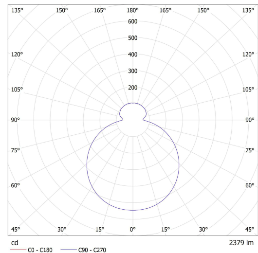
Lucis ZL3.K3.Z415 ZERO LED / LDC (Polar)
