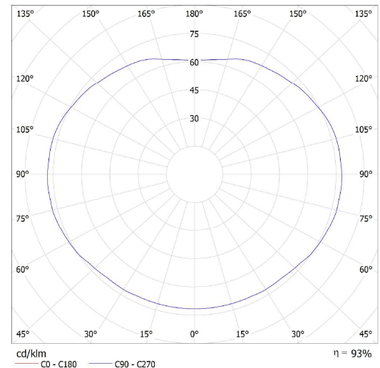
Lucis ZL1.11.400.X POLARIS ZL / LDC (Polar)
