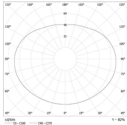
Lucis ZL1.11.300.X POLARIS ZL / LDC (Polar)
