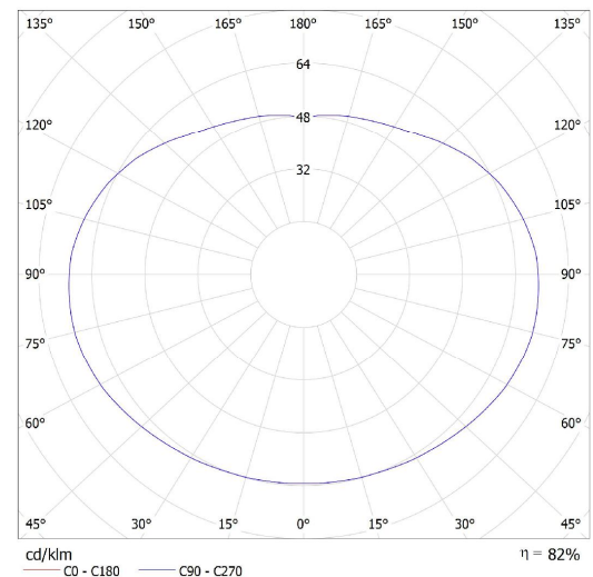
Lucis ZL1.11.300.X POLARIS ZL / LDC (Polar)
