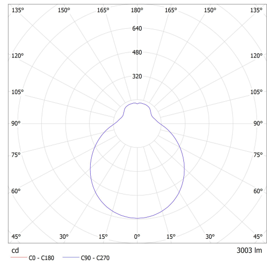
Luminaire: Lucis S37.L2.T14 CHARON LED Lamps: 1 x LED G6
