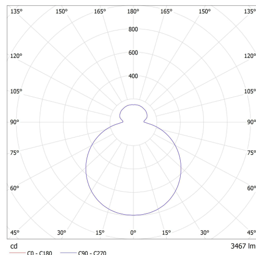
Luminaire: Lucis ZL3.K1.Z415 ZERO LED Lamps: 1 x LED G5
