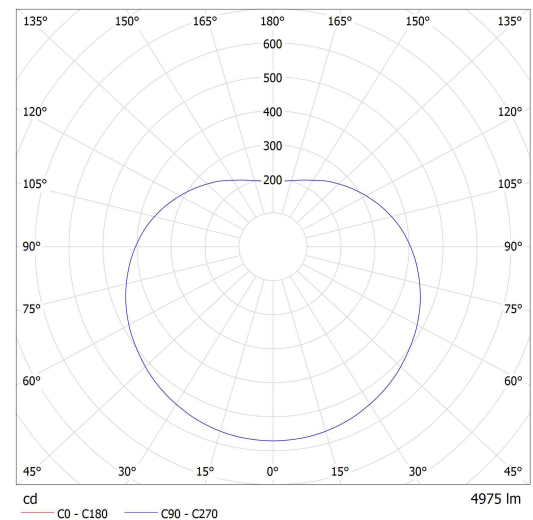
Lucis ZK.P1.500.X POLARIS ZK LED / LDC (Polar)
