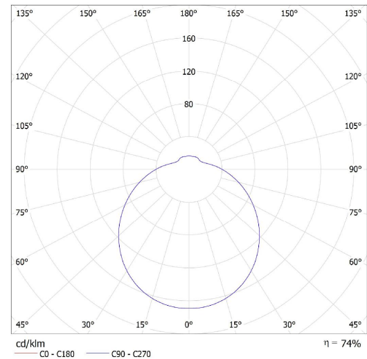
Lucis S33.112.CA3 CHARON PMMA / LDC (Polar)
