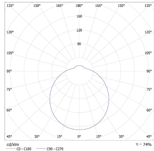
Lucis S26.111.CA2 CHARON PMMA / LDC (Polar)
