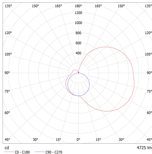
Lucis I1.L1.1200.X IZAR I LED / LDC (Polar)
