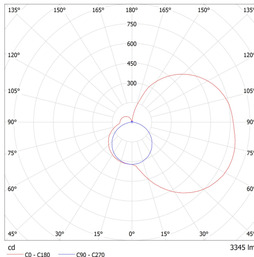
Lucis I1.L1.900.X IZAR I LED / LDC (Polar)
