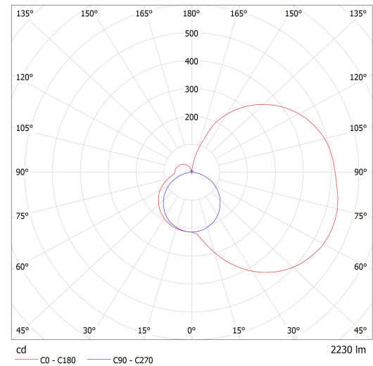
Luminaire: Lucis I1.L1.600.X IZAR I LED Lamps: 1 x LED G6
