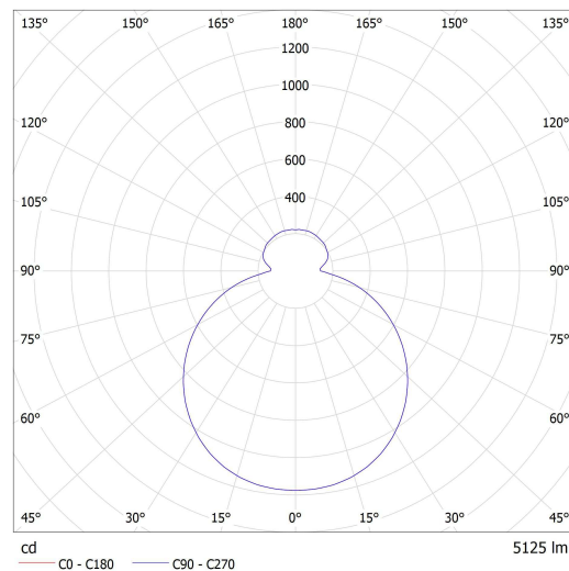
Lucis S46.K1.060 FORUM LED / LDC (Polar)
