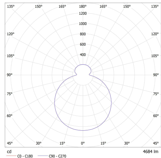
Luminaire: Lucis S43.K2.O50 FORUM LED Lamps: 1 x LED G5
