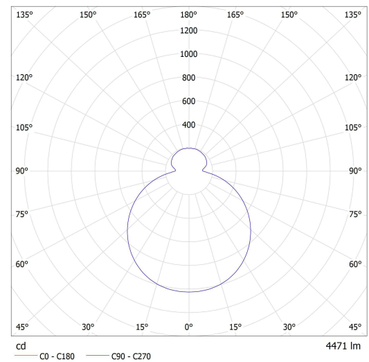
Lucis S43.K1.050 FORUM LED / LDC (Polar)
