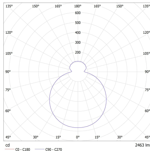
Lucis S34.K4.O42 FORUM LED / LDC (Polar)
