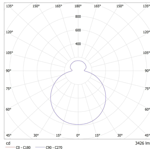
Lucis S34.K1.042 FORUM LED / LDC (Polar)
