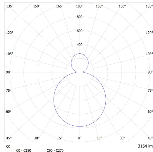
Lucis S34.K2.R550 RONDO LED / LDC (Polar)
